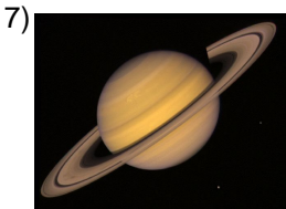
Saturn
