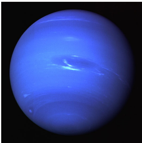
Neptune
