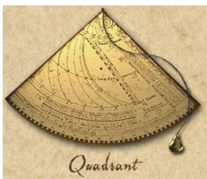
quadrant
