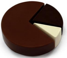
to divide
