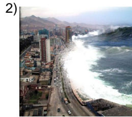
tsunami
