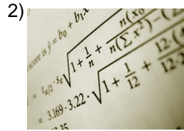
statistics
