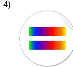
equal
