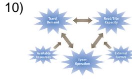
factors
