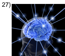
brain
