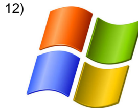
operating system
