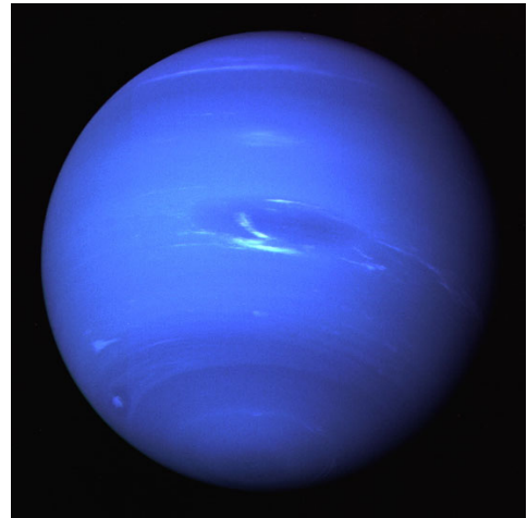
Neptune
